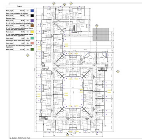
*Line drawing
